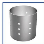
Bucket(optional)
